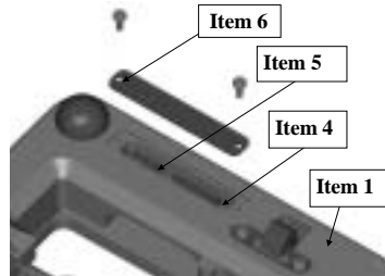
Figure 5: Pin storage
