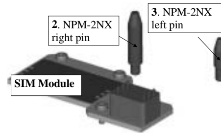
Figure 4: Parts needed for NPM-2NX.
